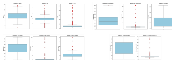
Figure 3. Boxplot Visualization
