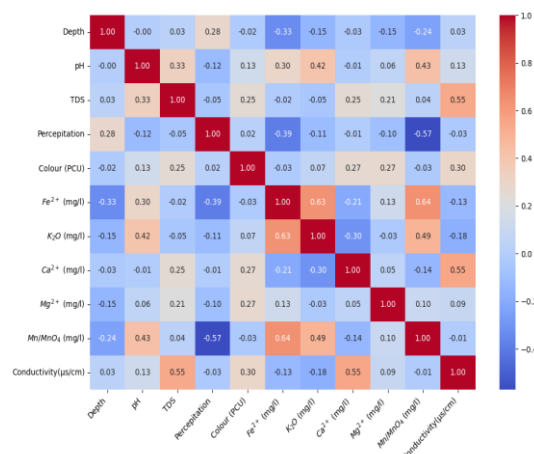
Figure 2. Heatmap Visualization
