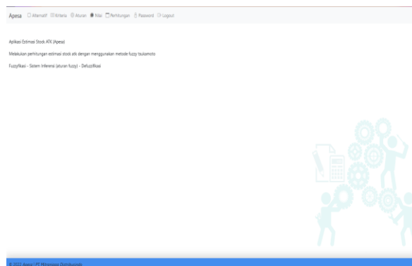
Figure 9. Dashboard Page
