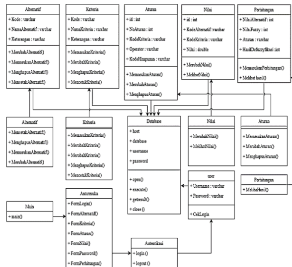
Figure 6 Class Diagram
