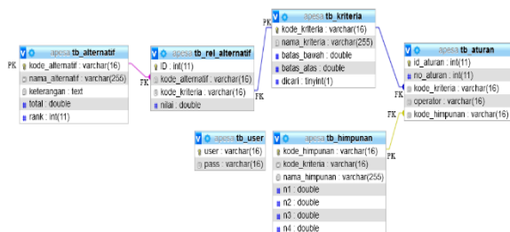
Figure 8 Database Relationship
