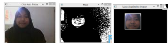
Figure 8. Face Detection
