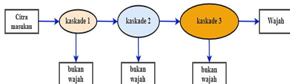
Figure 5. Graded Classification Flow
