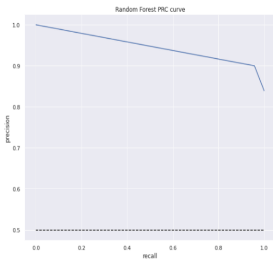
Figure 12. PRC Random Forest
