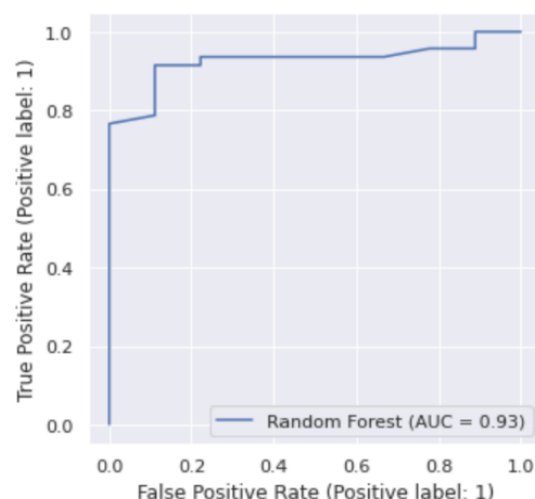
Figure 11. AUC Random Forest
