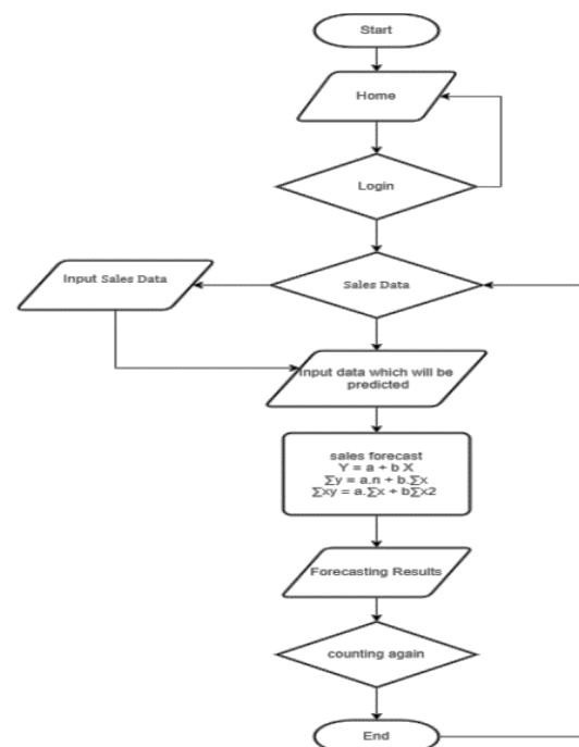
Figure 4. Algorithm Trend Moment
