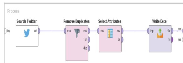
Figure 2. Tweet Data Crawling Model Design
