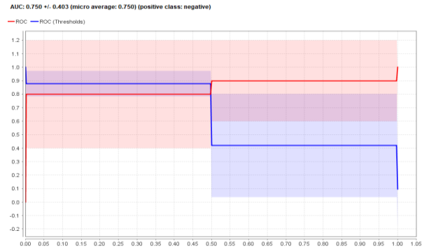
Figure 9. ROC Fund Sentiment Curve using NBC + PSO
