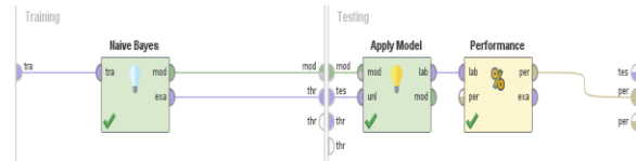
Figure 6. Design of Sentiment Classification Model iSaku uses the Naïve Bayes Classifier
