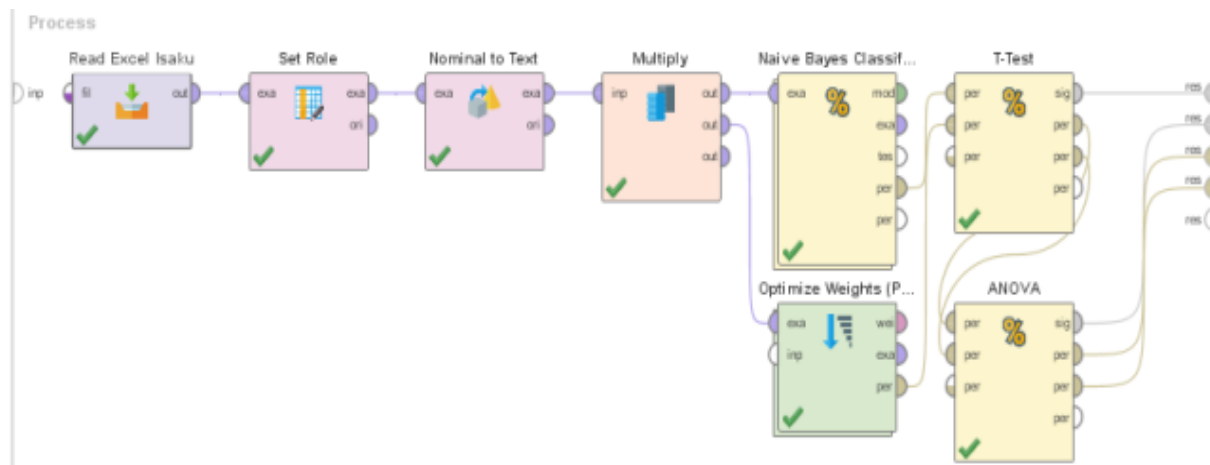
Figure 13. Design of the T-Test and Anova Model Test for Classification of NBC with NBC + PSO Sentiment iSaku
