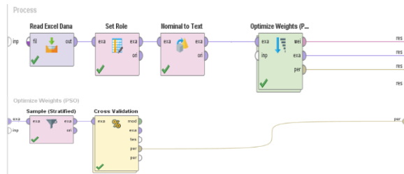
Figure 8. Design of a Fund Sentiment Model using NBC + PSO
