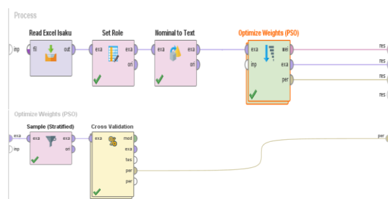
Figure 10. Design of Sentiment Model iSaku uses NBC + PSO
