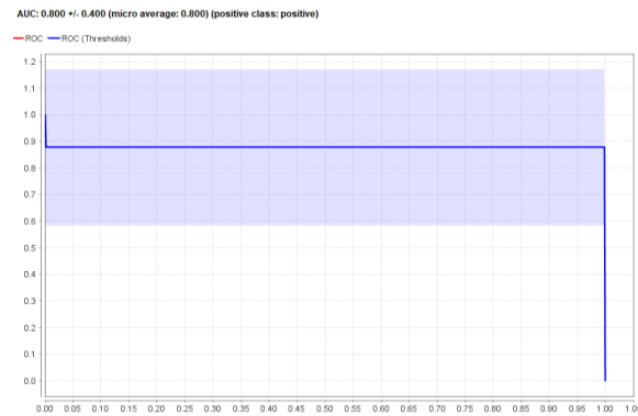
Figure 11. ROC Sentiment Curve iSaku using NBC + PSO
