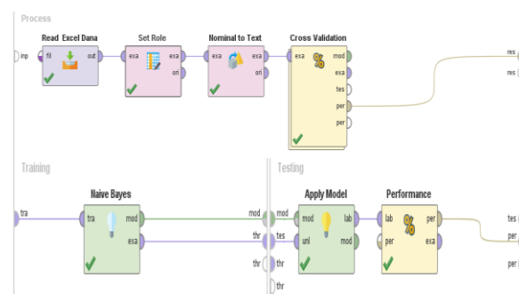
Figure 4. Design of Sentiment Classification Model Funds using the Naïve Bayes Classifier
