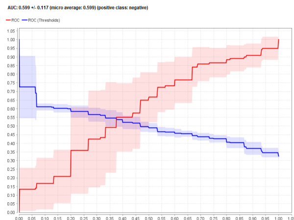
Figure 5. ROC Fund Sentiment Curve using the Naïve Bayes Classifier
