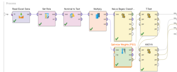
Figure 12. T-Test Model Design and Anova Model Classification of NBC with NBC + PSO Fund Sentiment
