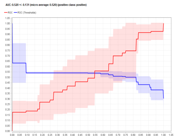
Figure 7. ROC Sentiment Curve iSaku using the Naïve Bayes Classifier
